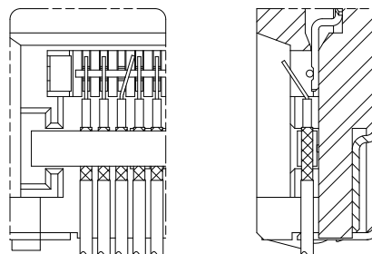
① Misalignment in pitch direction
