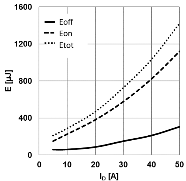
Figure 16 Typical switching energy losses as a function of drain-source current (E = f(I_{DS}), V_{DD} = 800\text{V}, V_{GS} = 0\text{V}/15\text{V}, R_{G,ext} = 2\Omega, T_{vj} = 175^{\circ}\text{C}, \text{ind. load, test circuit in Fig. E, diode: body diode})
