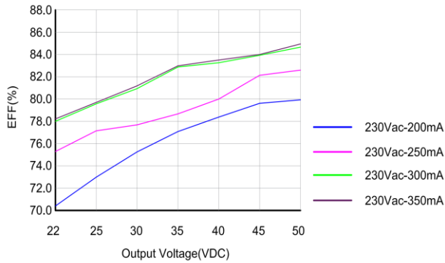
Efficiency VS.Load
