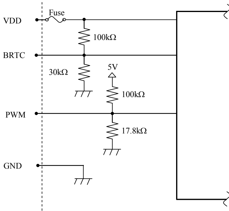
LED driver circuit
