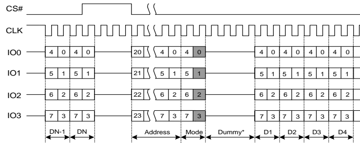
Figure 7.20 Fast Read Quad I/O Instruction(Previous command set M5-4 = 10)
