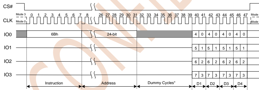
Figure 7.16 Fast Read Quad Output Instruction
