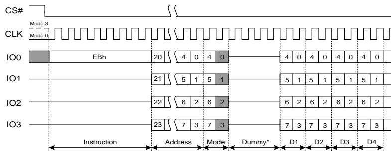
Figure 7.19a Fast Read Quad I/O Instruction(Initial command or previous M5-4 ≠10)
