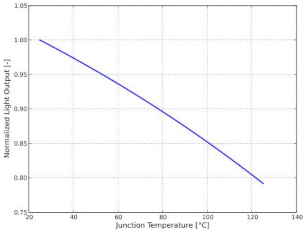
Figure5. Typical normalized light output vs Junction temperature
