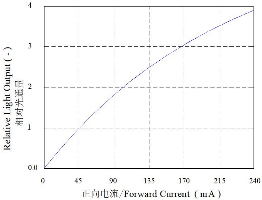
Figure4. Typical normalized light output vs. forward current
