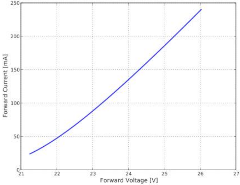
Figure3. Typical forward current VS forward voltage
