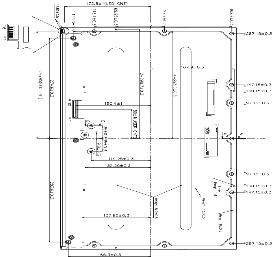
Figure 6. TFT-LCD Module Outline Dimensions (Rear view)
