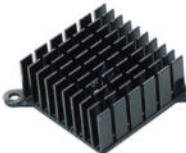
Model:AK-HS-38 Size:37*37*17mm
