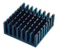
Model:AK-HS-34 Size:25*25*10mm
