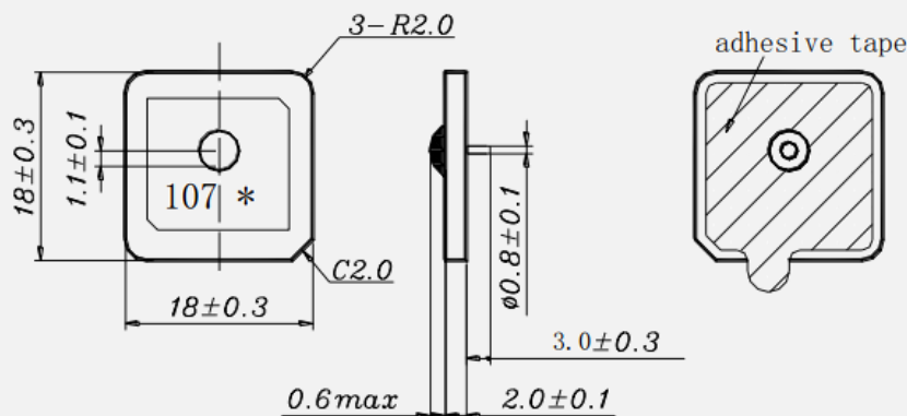
Figure 2 Dimensions
