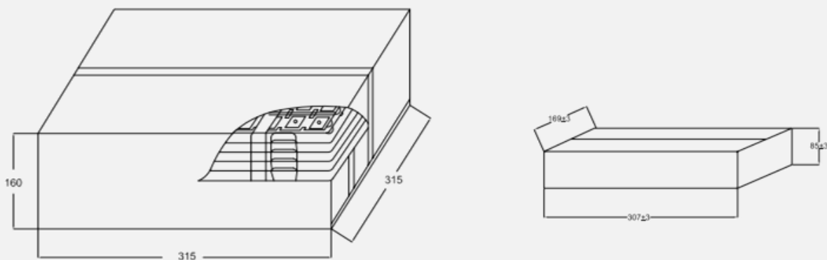
Figure 8 PACKING
