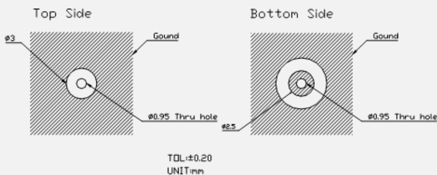
Figure 3 Layout Dimensions
