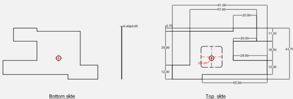
Figure 5 Ground Plane
