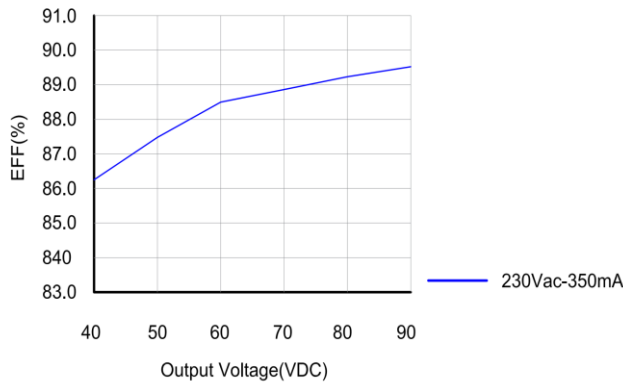
Efficiency VS.Load
