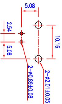
PC BOARD LAYOUT
