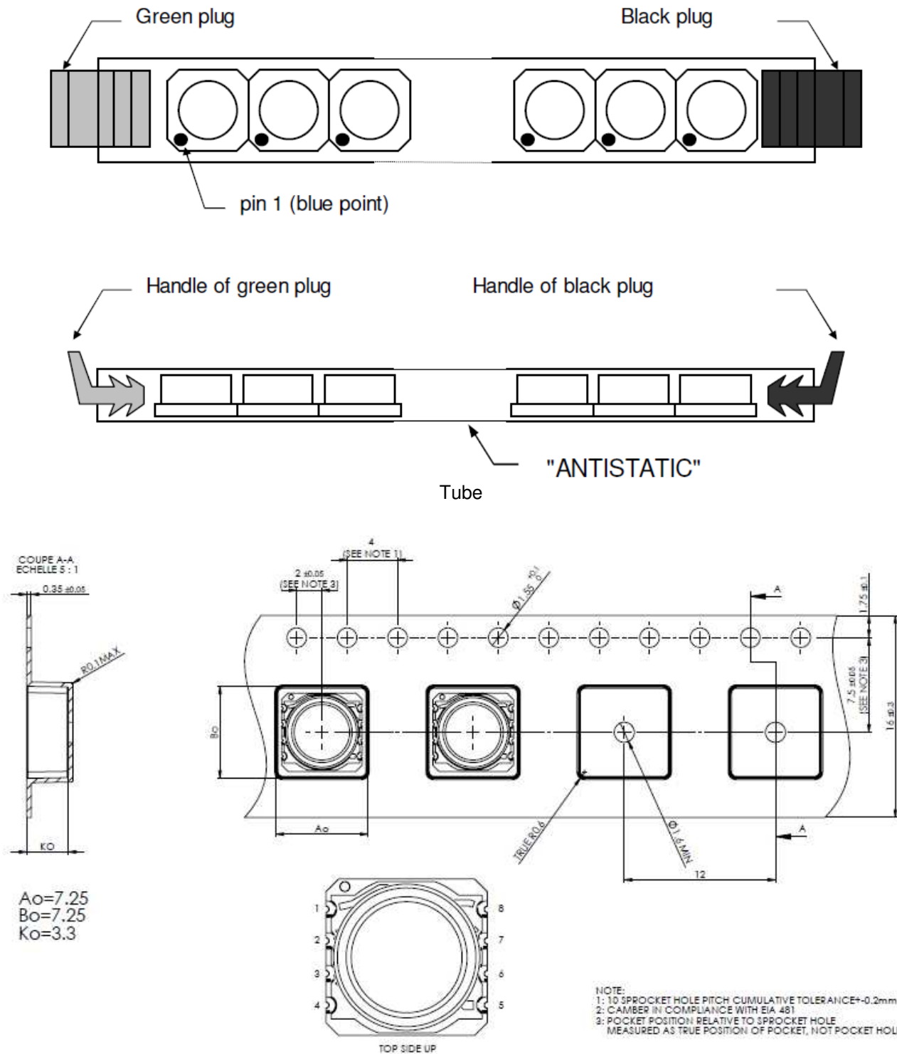
Tape & reel
