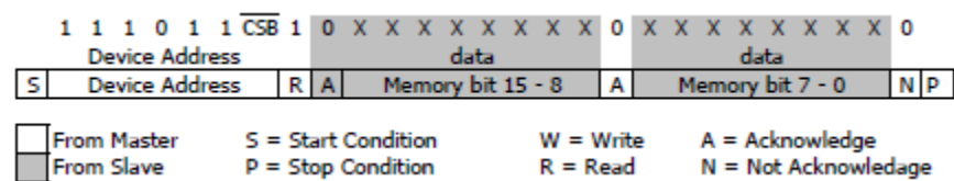
Figure 12: I 2 C answer from MS5803-01BA
