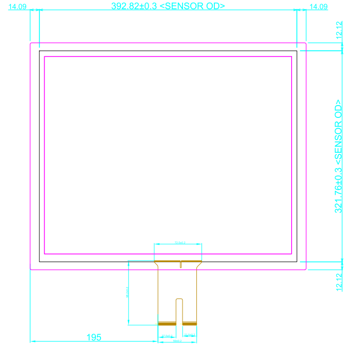
Back View
