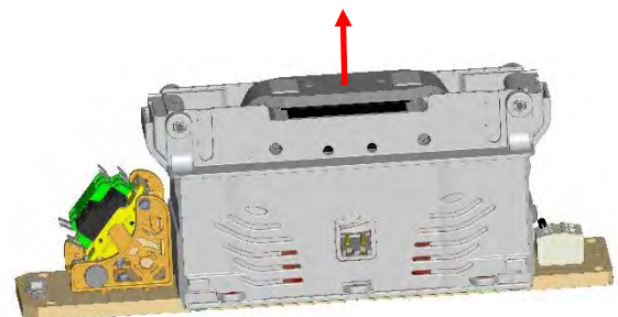
Contact carrier, for CT1115/08 V and CT1130/08 V
