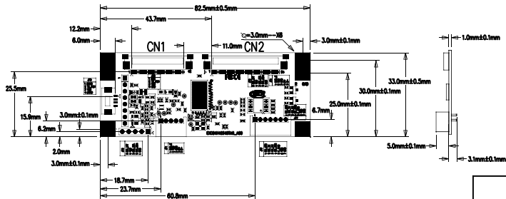
Scale 2 : 1 Control board
