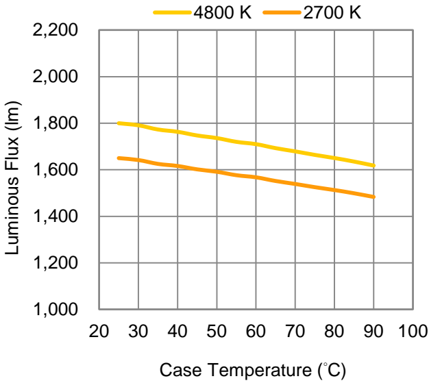
Fig 4. Case Temperature vs. Luminous Flux at 450 mA.
