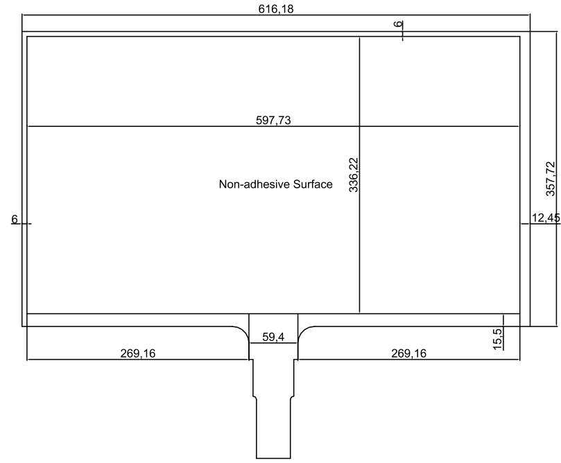
Golden Finger FRONT Effective width:597.73;Effective height:336.22;Cutting width:616.18;Cutting height:357.72
