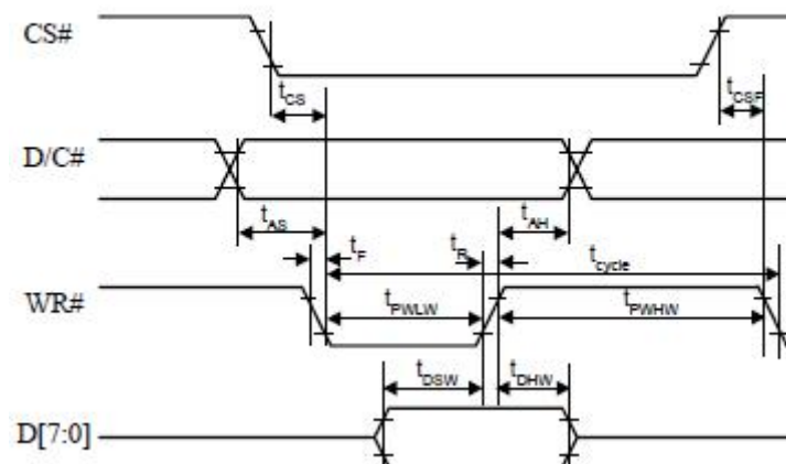
Write Cycle
