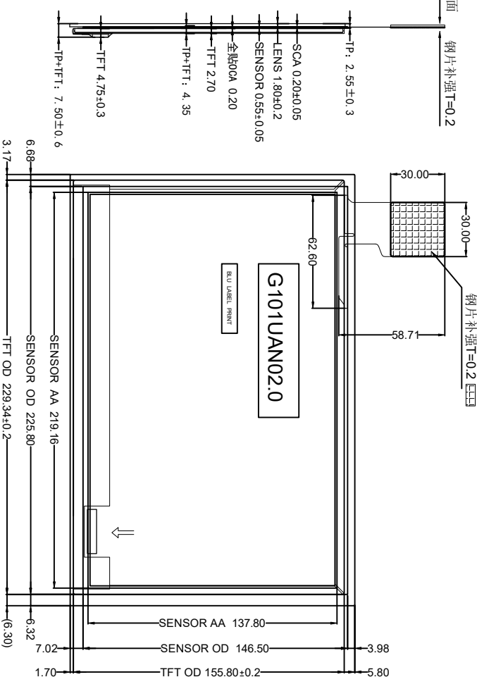
Side View
