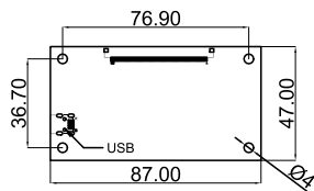
STM Controller
