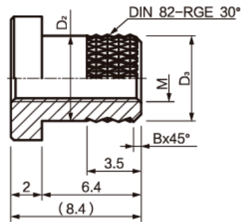
Diamond knurling
