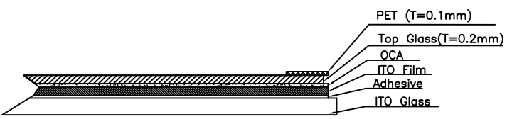
DETAIL A
