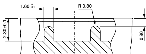
Section "A" (IC-595-1 only)
