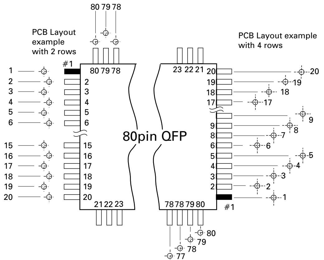
QFP package possible positions for Pin #1.
