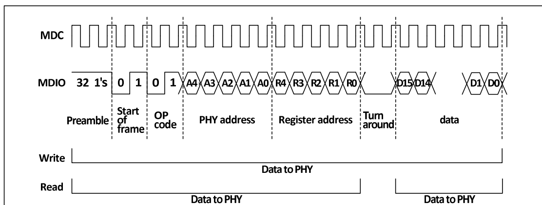
Figure 27-3 SMI Interface read and write speed diagram
