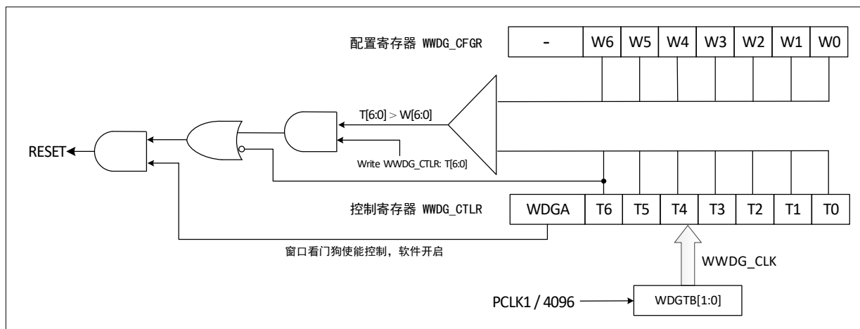
Figure 8-1 Window Watchdog block diagram
