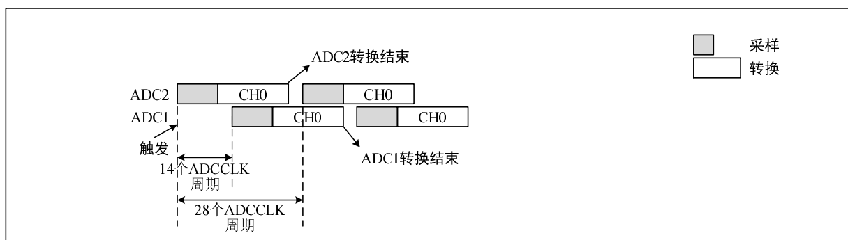
Figure 12-9 Slow interleaved mode on 1 channel
