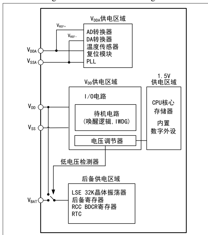
Figure 2-1 Power structure diagram
