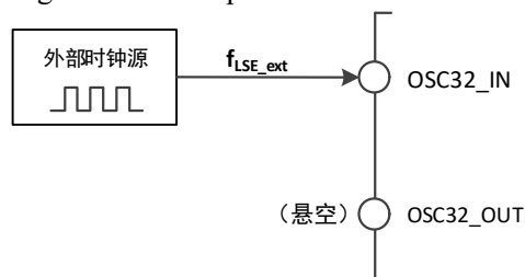
Figure 3-9 Low-speed clock source circuit
