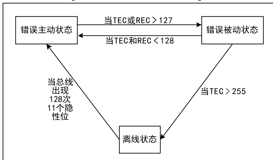
Figure 24-6 CAN error state switch diagram
