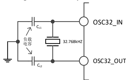
Figure 3-8 LSE crystal circuit
