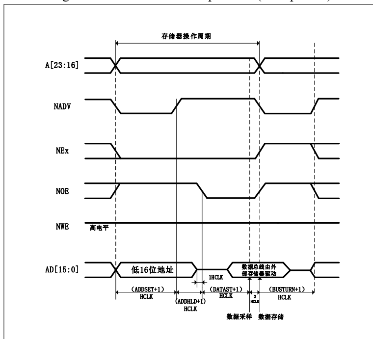
Figure 26-11 Mode D read operation (multiplexed)
