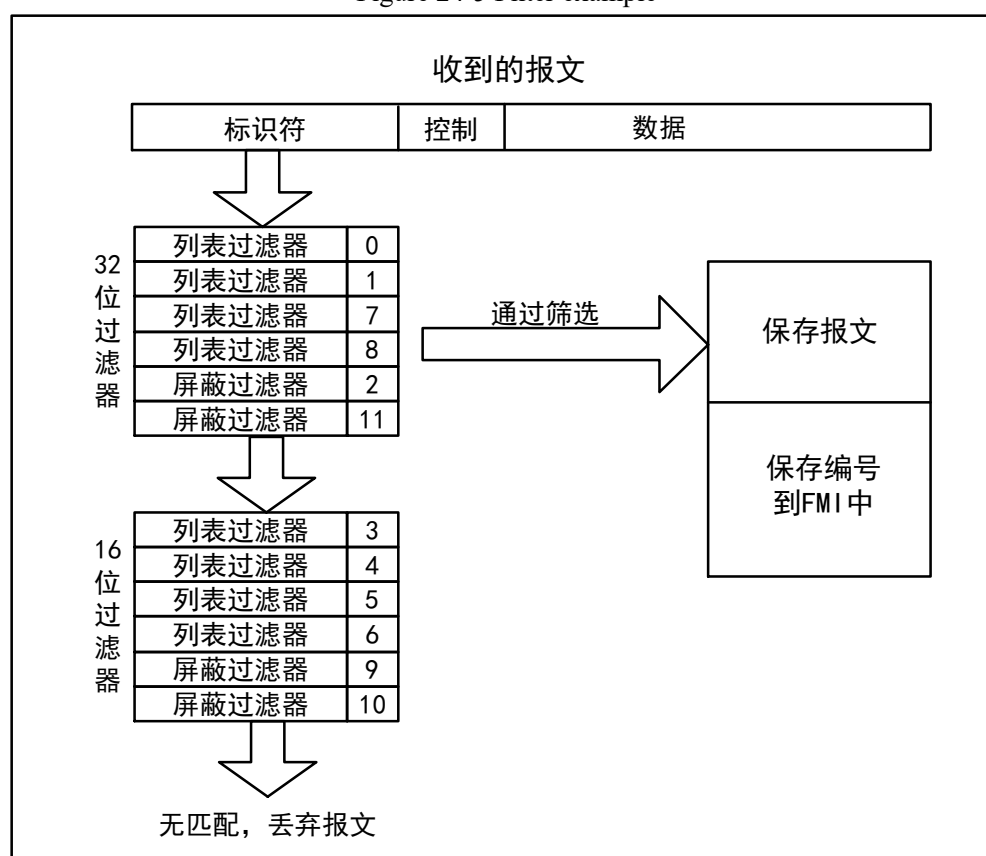
Figure 24-5 Filter example
