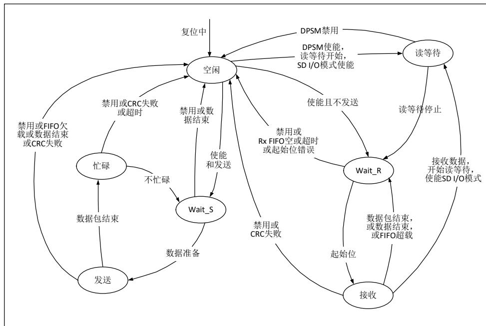
Figure 28-3 Data path state machine
