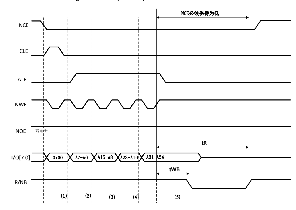
Figure 26-16 Special operation on NAND FLASH
