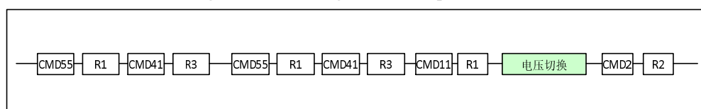
Figure28-13 Voltage switch sequence
