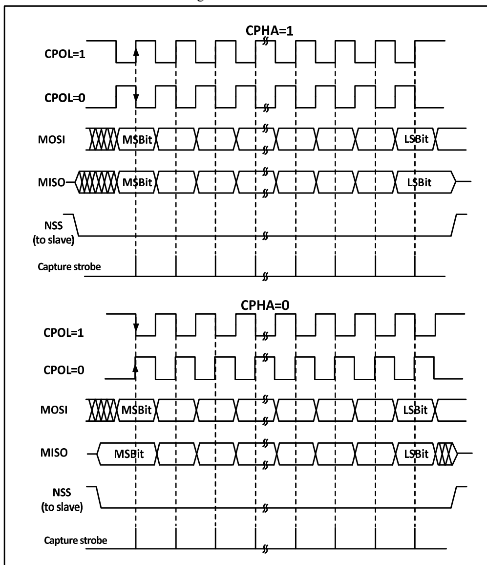
Figure 20-2 SPI model
