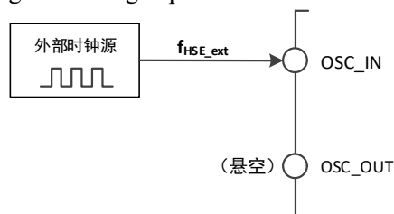
Figure 3-7 High-speed clock source circuit
