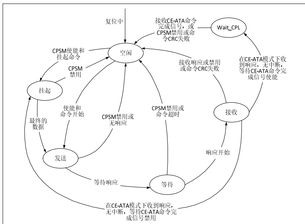
Figure 28-2 Command path state machine
