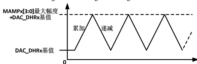
Figure 17-4 Triangular wave generation
