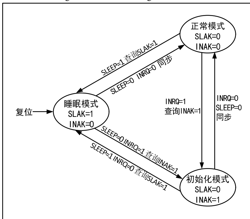
Figure 24-1 CAN working mode switch
