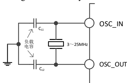
Figure 3-6 HSE crystal circuit
