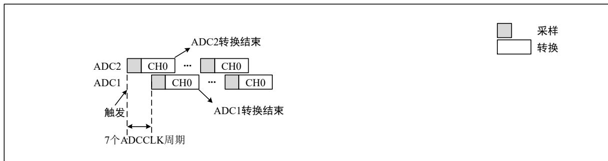
Figure 12-8 Fast interleaved mode on 1 channel in continuous conversion mode
