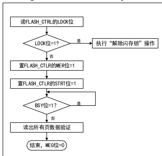
Figure 32-3 FLASH Full chip erase
