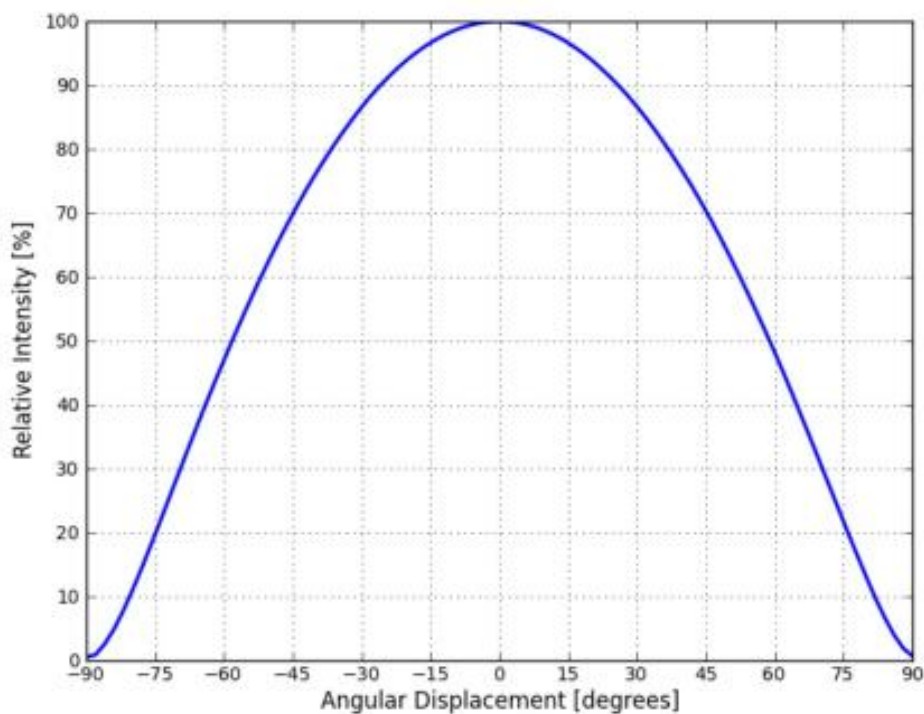
Figure7.Typical radiation patten
