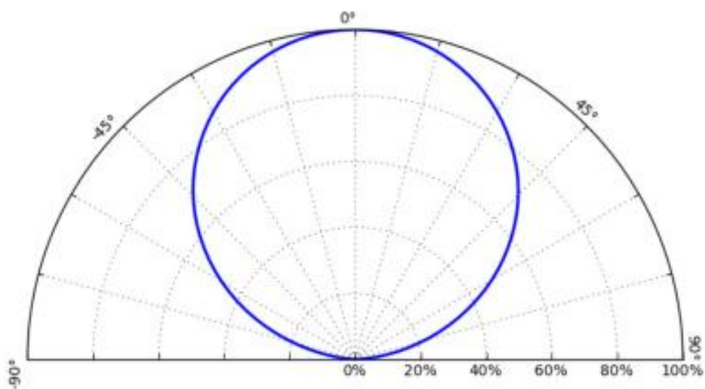
Figure8.Typical polar radiation pattern
