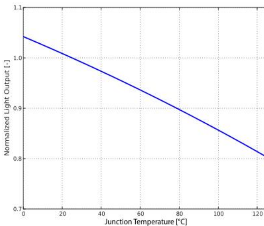
Figure6. Typical normalized light output vs Junction temperature
