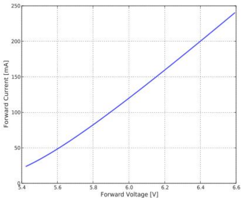
Figure4. Typical forward current VS forward voltage
