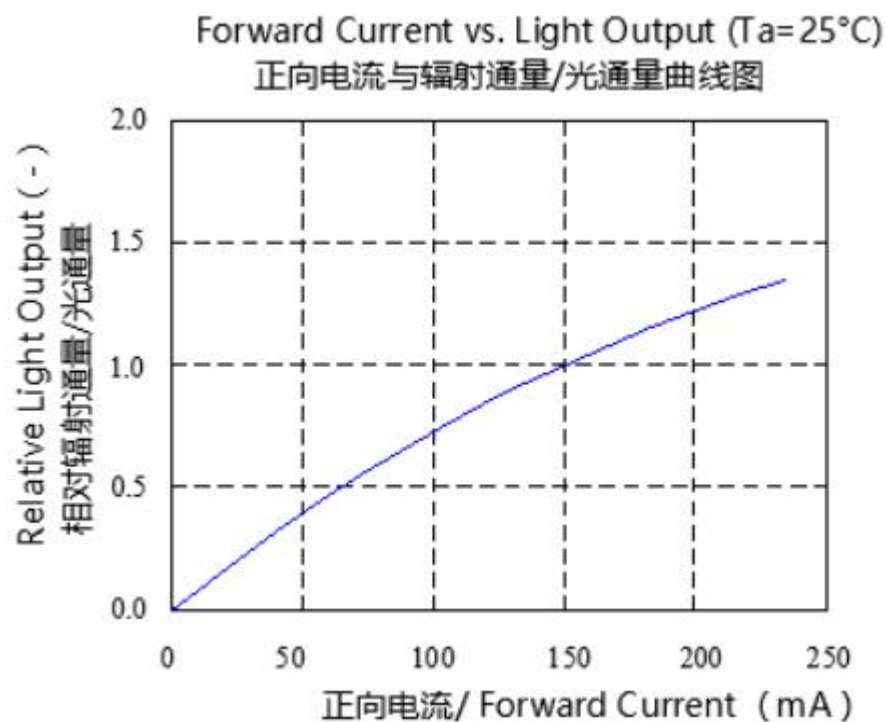
Figure5. Estimated typical ratio compared to flux at rated condition
