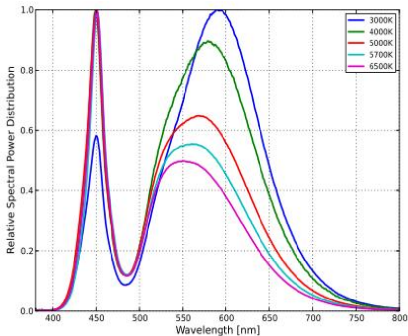
Figure1. Typical Color Spectrum for 70CRI
