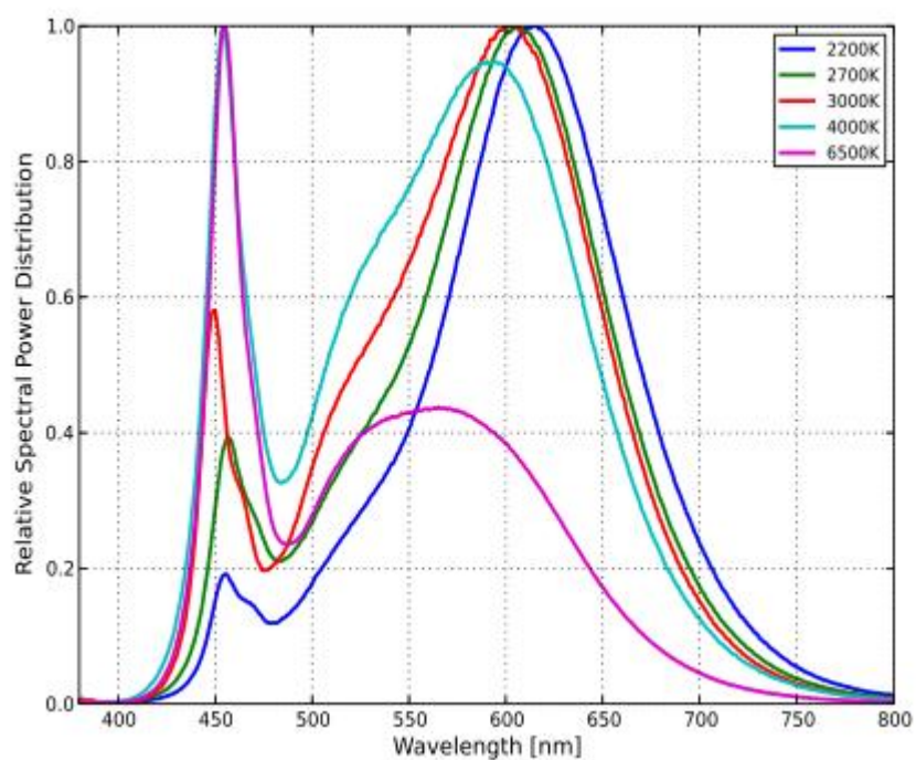
Figure2. Typical Color Spectrum for 80CRI
