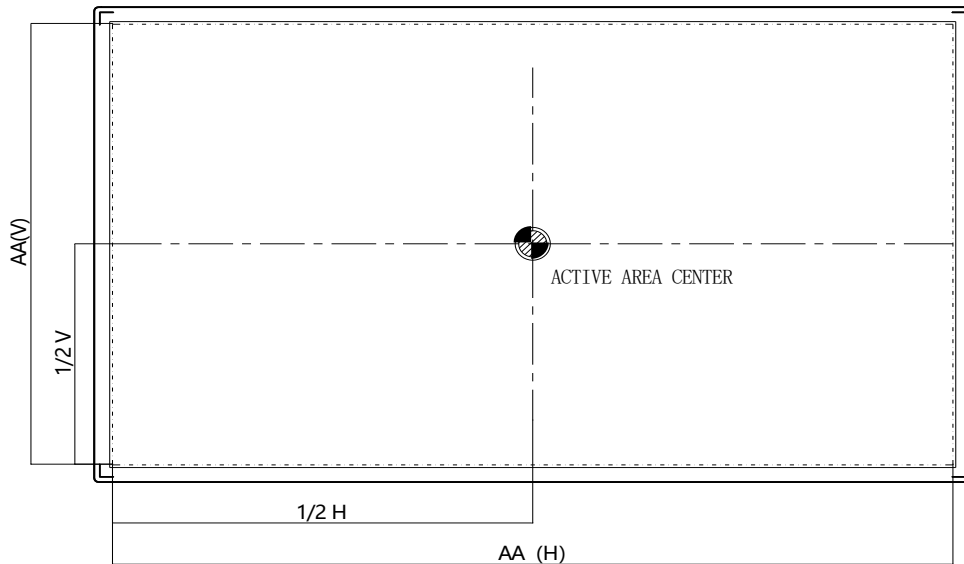
< Figure 5. White Luminance and Uniformity Measurement Locations >
