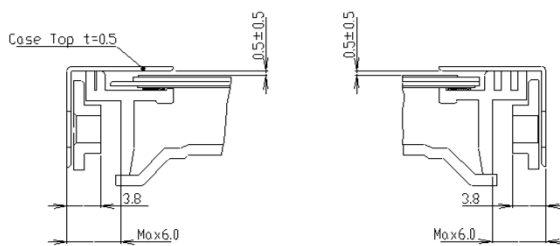
SECTION A-A SCALE 2/1
