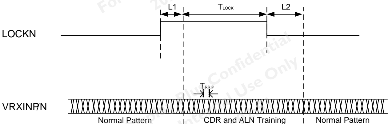
1. V-by-one Signal diagram
