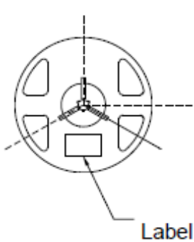
Fig.2-2 Reel Dimension
