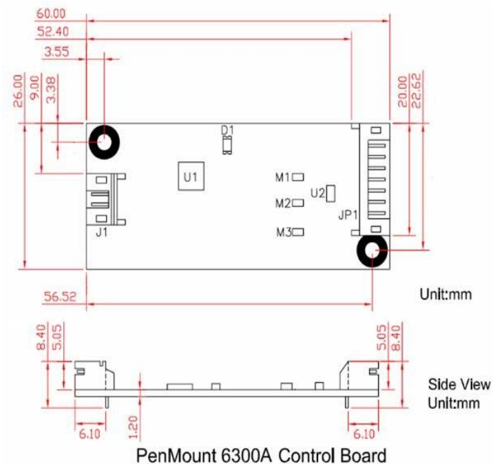
PenMount 6300A Touchscreen Control Board Mechanical Diagram
