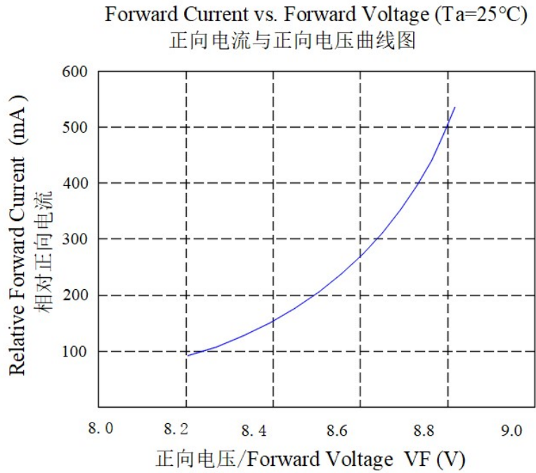
Figure3. Typical forward current VS forward voltage
