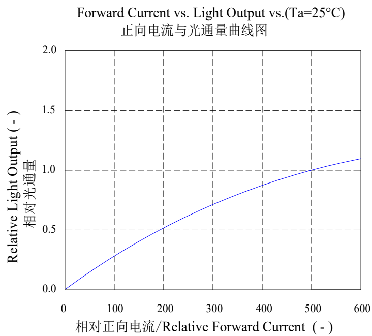
Figure4. Typical normalized light output vs. forward current
