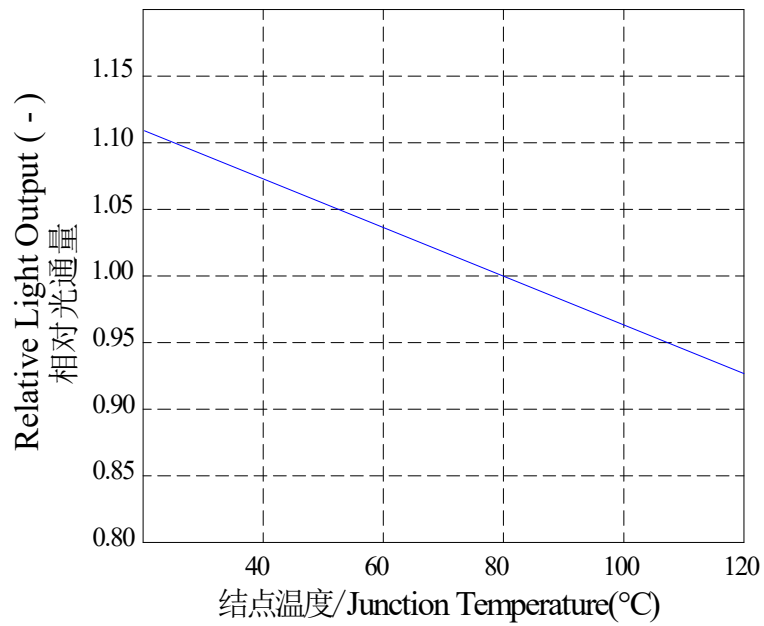
Figure5. Typical normalized light output vs Junction temperature
