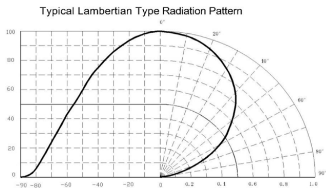
Radiation diagram
