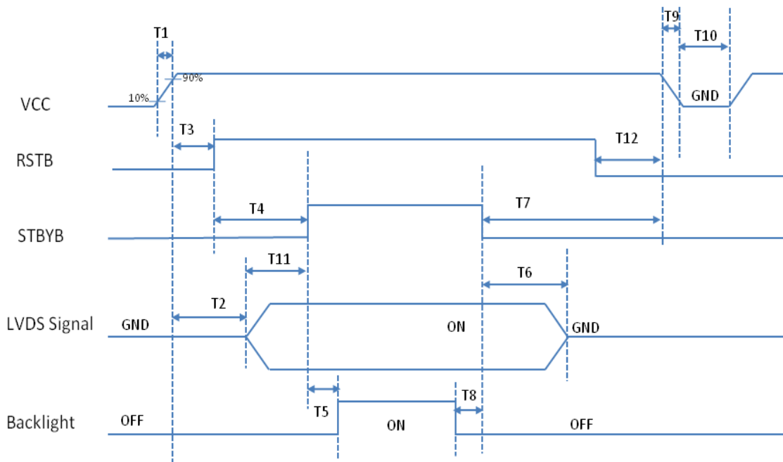
Figure 19 Power Sequence
