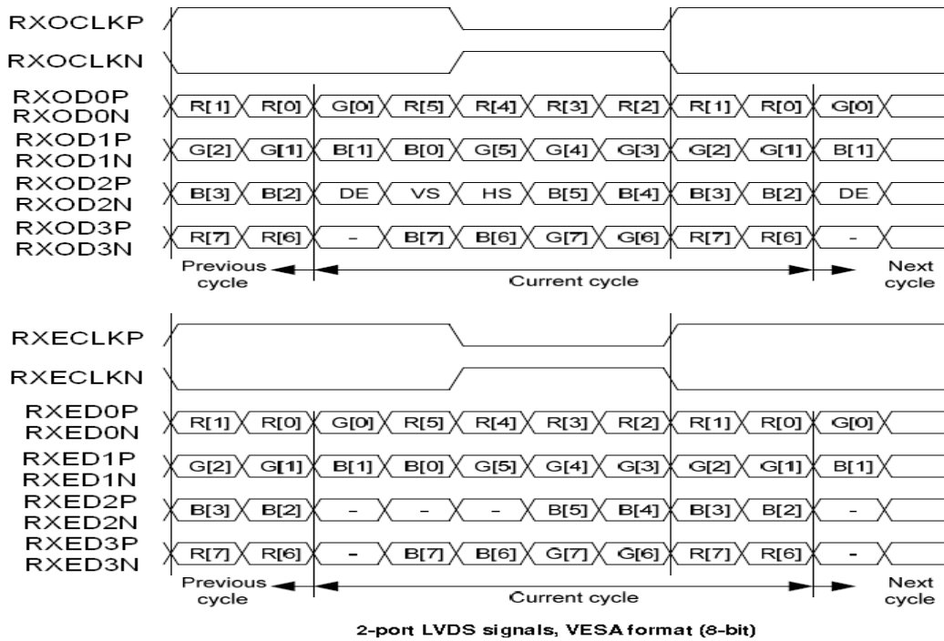
Figure 14 Data Mapping
