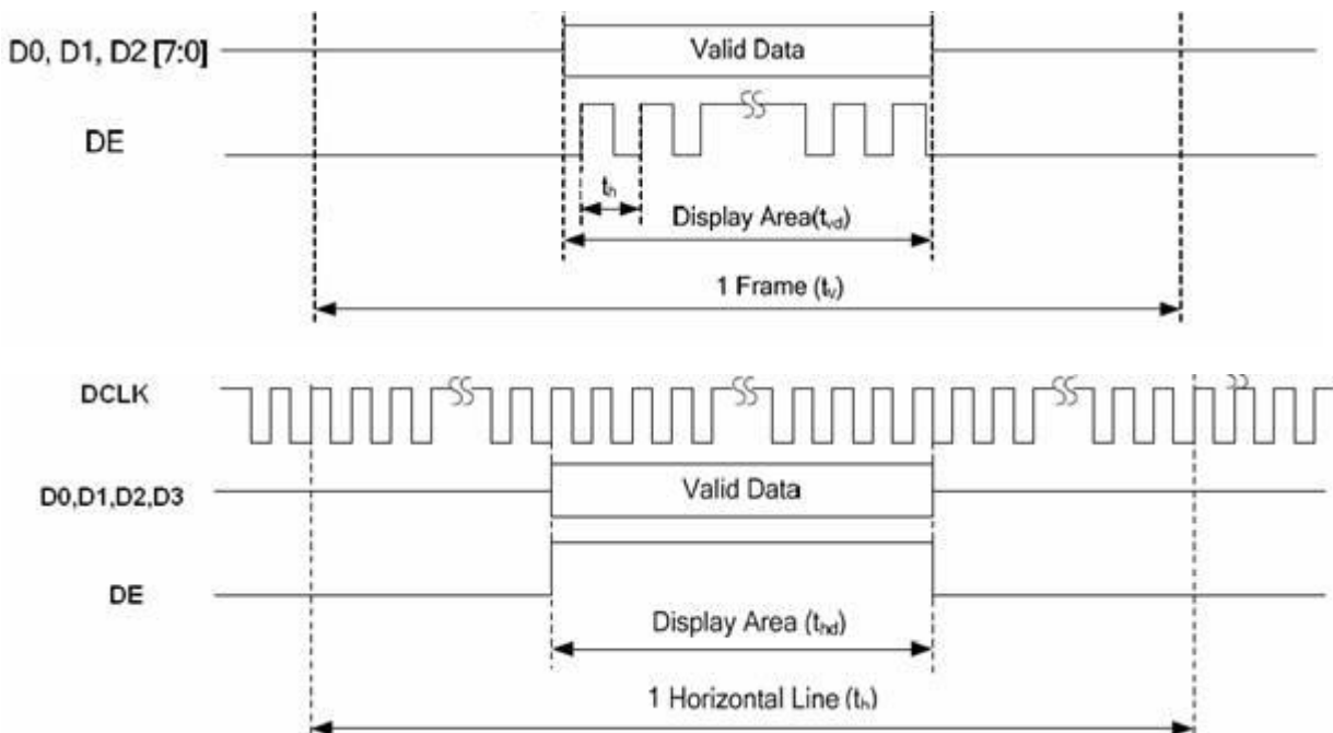
Figure 16 Timing Diagram
