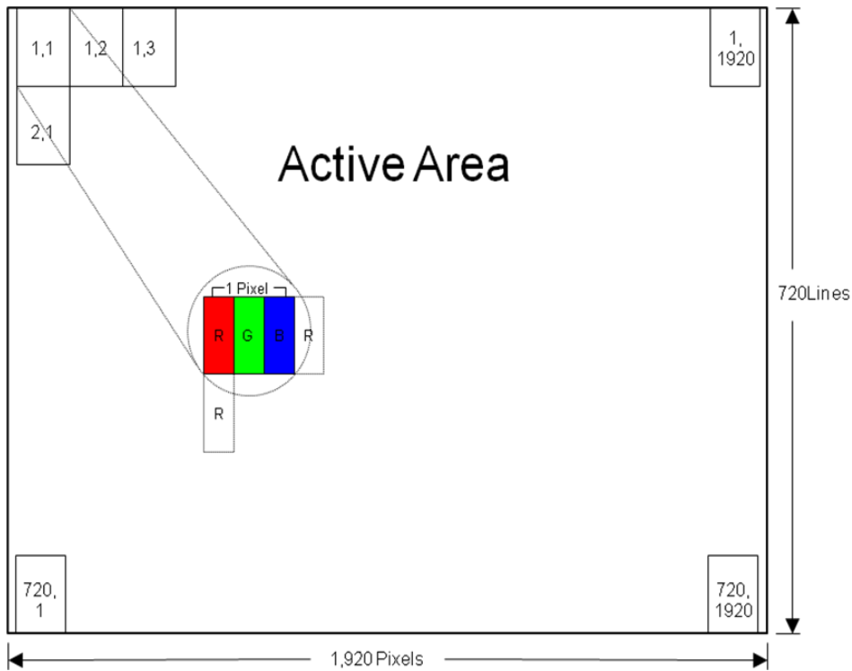
Figure 2 Pixel Mapping
