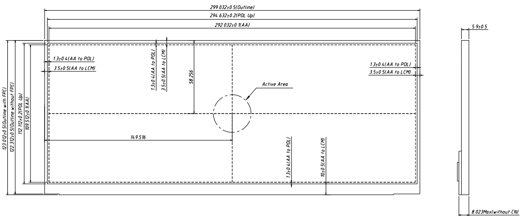
Figure 20 Reference Outline Drawing (Front Side)
