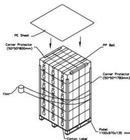
Figure. 9-2 Packing method
