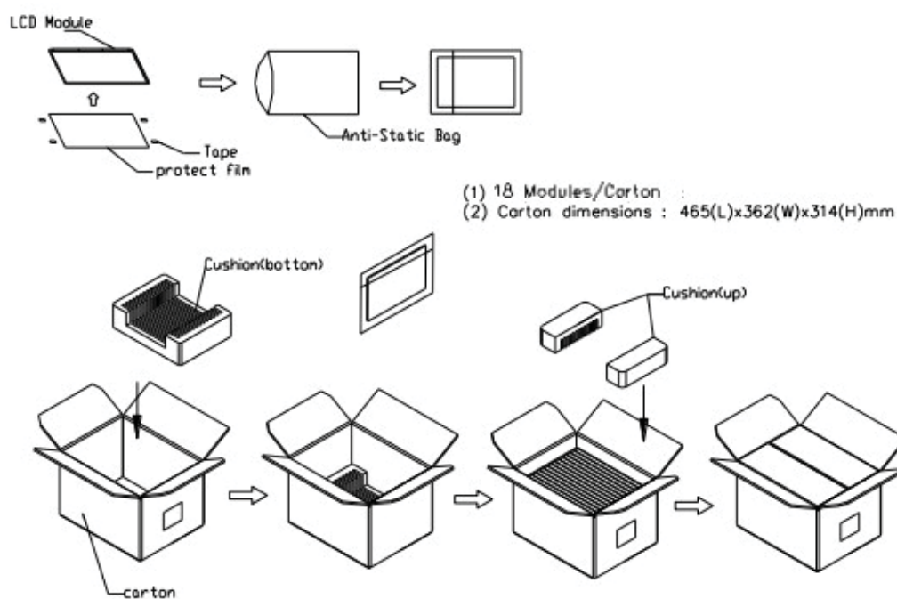
Figure. 9-1 Packing method
