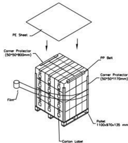
Figure. 9-2 Packing method
