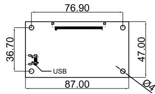
STM Controller
