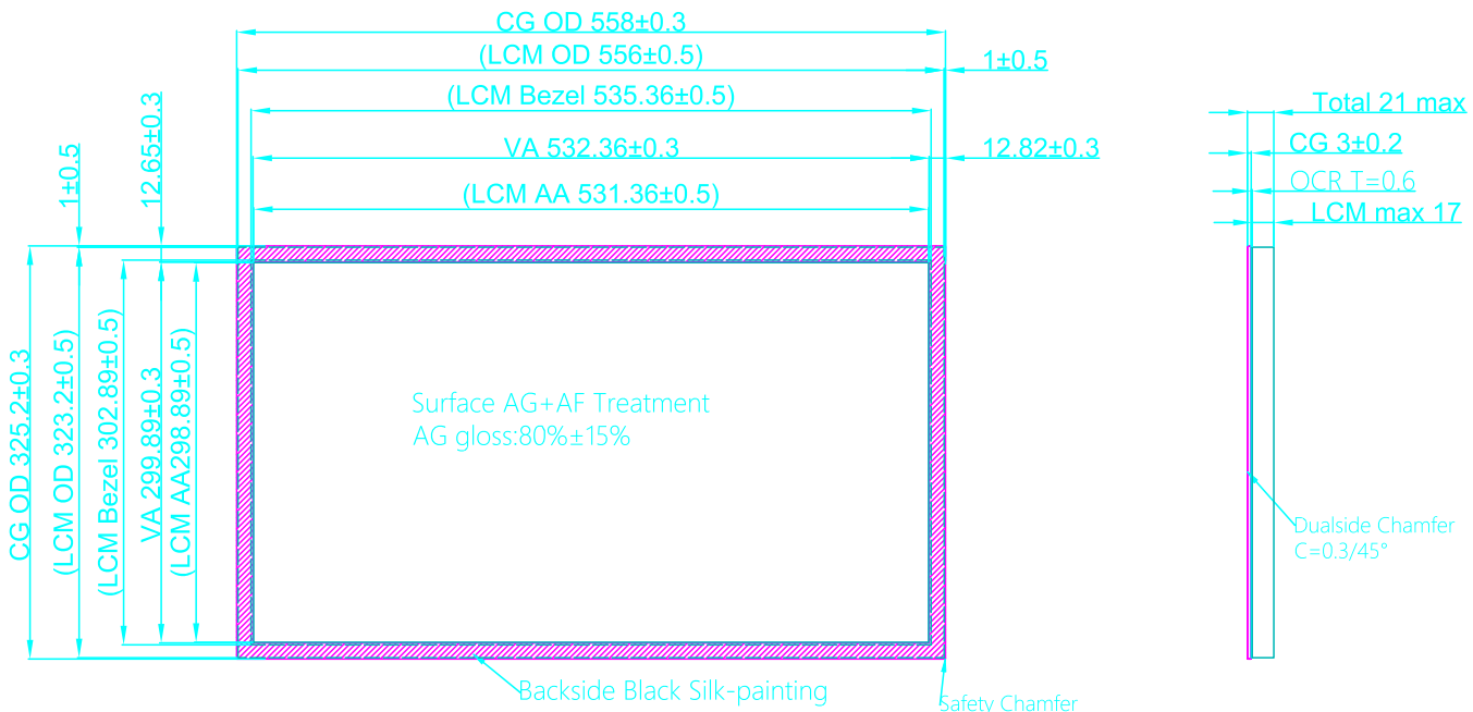
Front view
