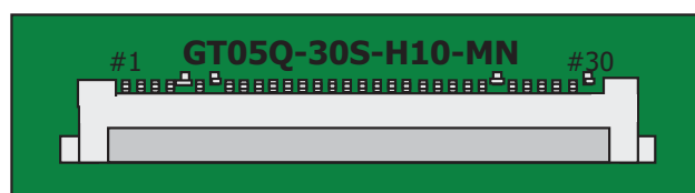
FIG.4 Connector diagram
