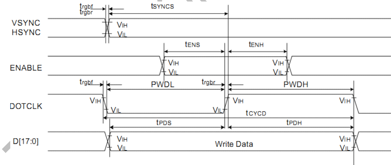
Figure 5.3 Parallel 18/16/6-bit RGB Interface Timing Characteristics
