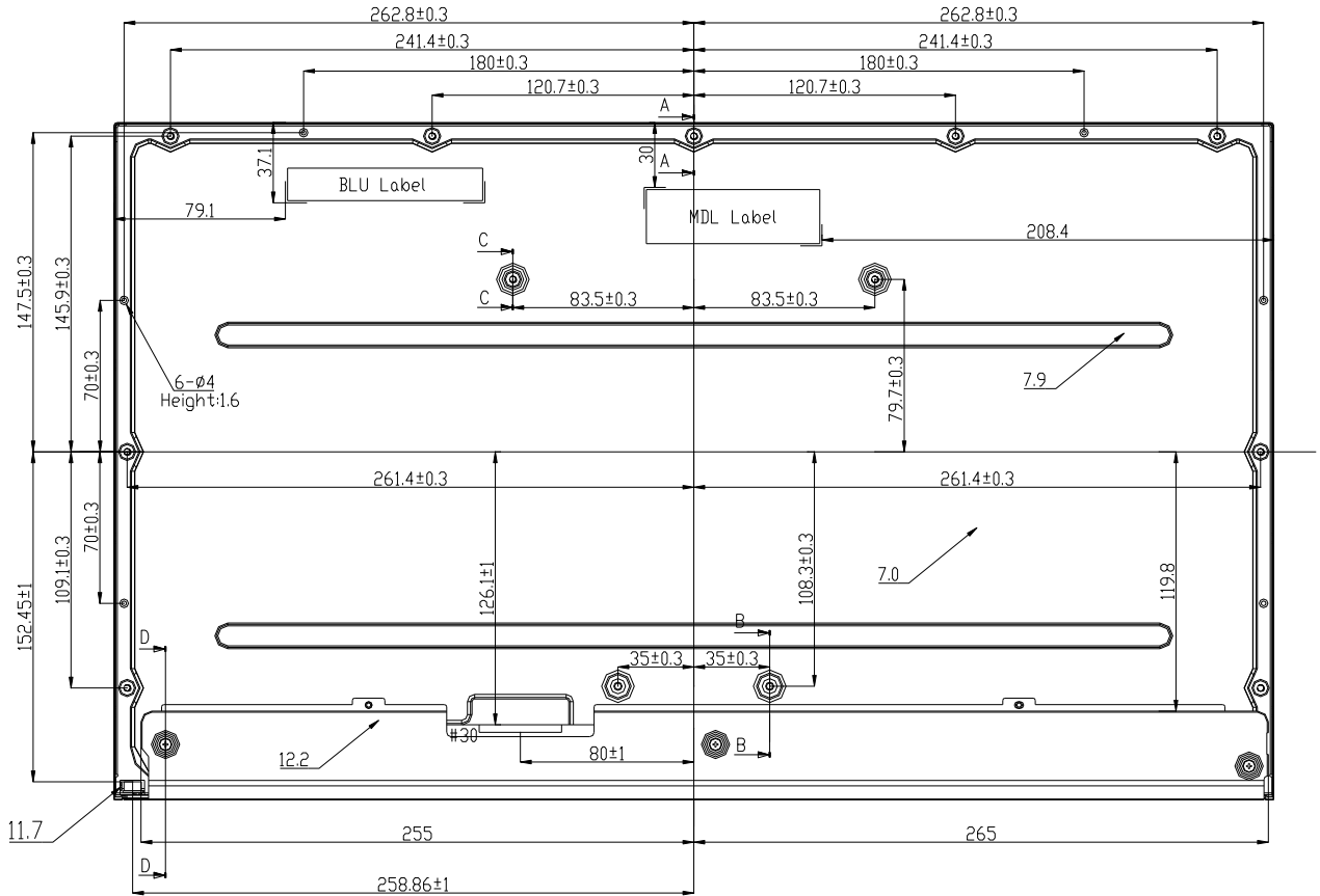
Figure 6. TFT-LCD Module Outline Dimensions (Rear view)
