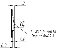
Section C-C Scale 2:1
