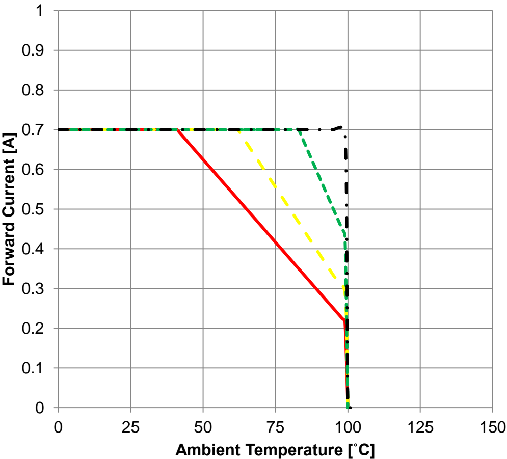
Derating Curve:
