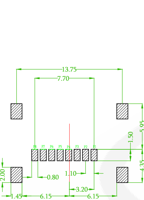
RECOMMENDED PCB LAOUT (PCB TOLERANCE ±0.05)
