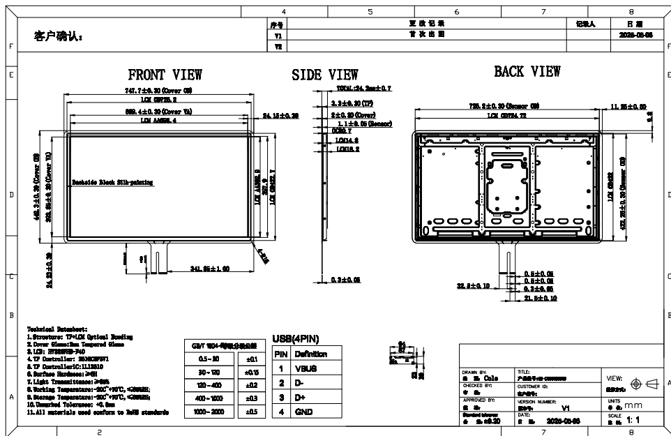
TP+LCM optical bonding drawing
