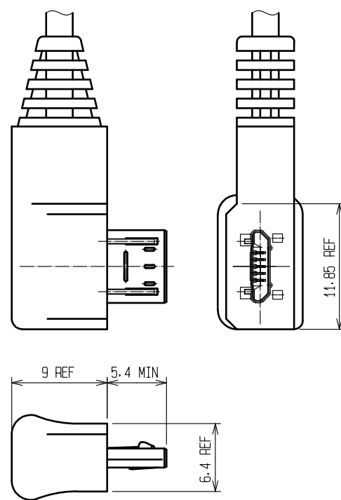
Fig-3 OVER-MOLDING(REFERENCE)
