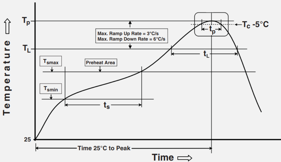
Figure 9 Reflow soldering profile (Refer to IPC/JEDEC J-STD-020E)
