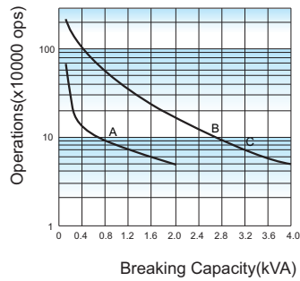
ENDURANCE CURVE
