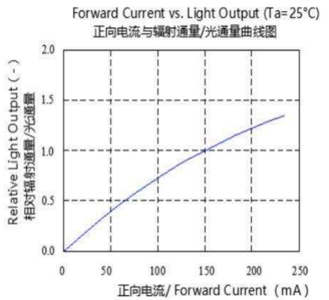
Figure5. Typical ratio compared to flux at rated condition
