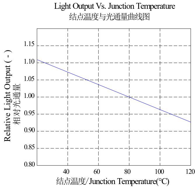
Figure6. Typical normalized light output vs Junction temperature
