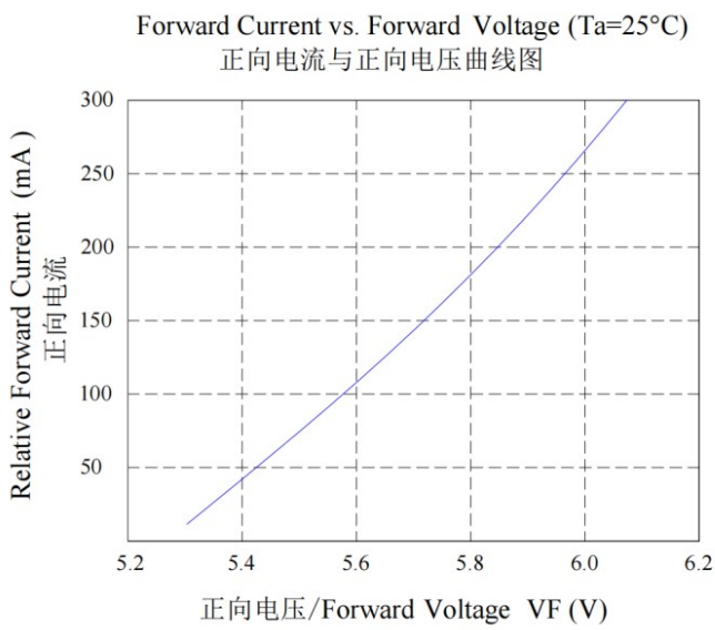
Figure4. Typical forward current VS forward voltage
