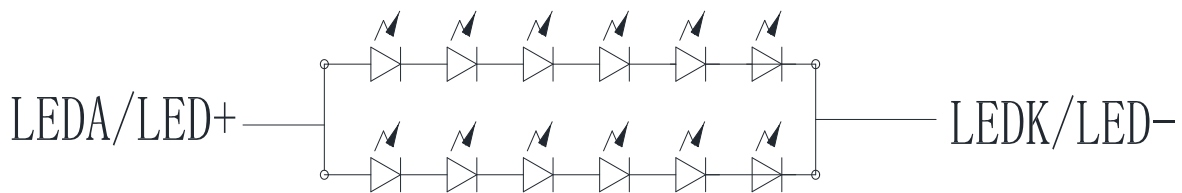
CIRCUIT DIAGRAM
