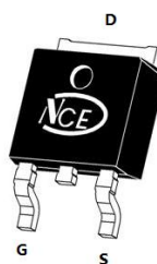
TO-252
