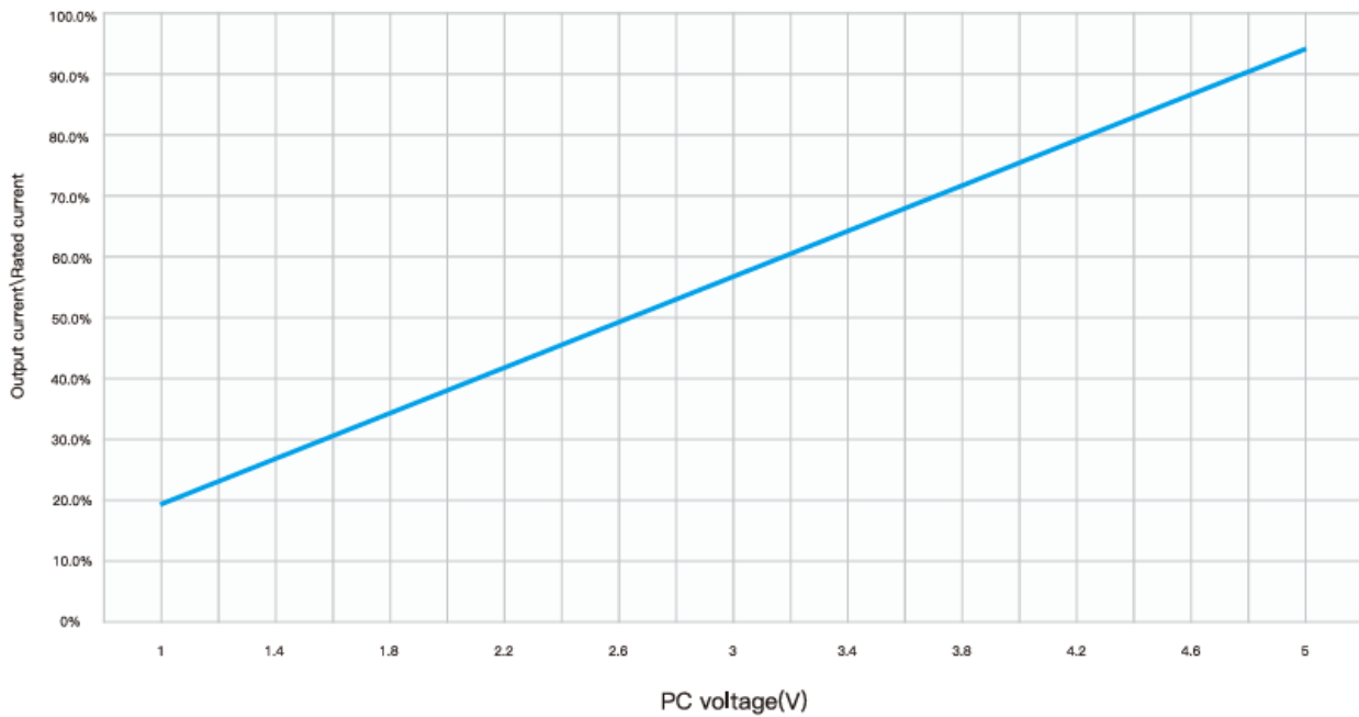
Output voltage vs PC voltage
