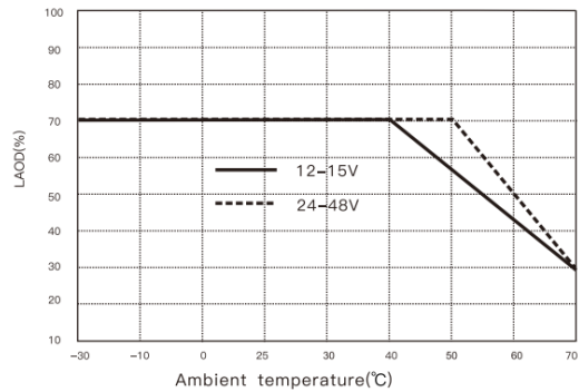
Derating curve (convection cooling)
