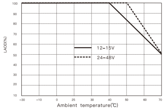
Derating curve (forced air cooling)
