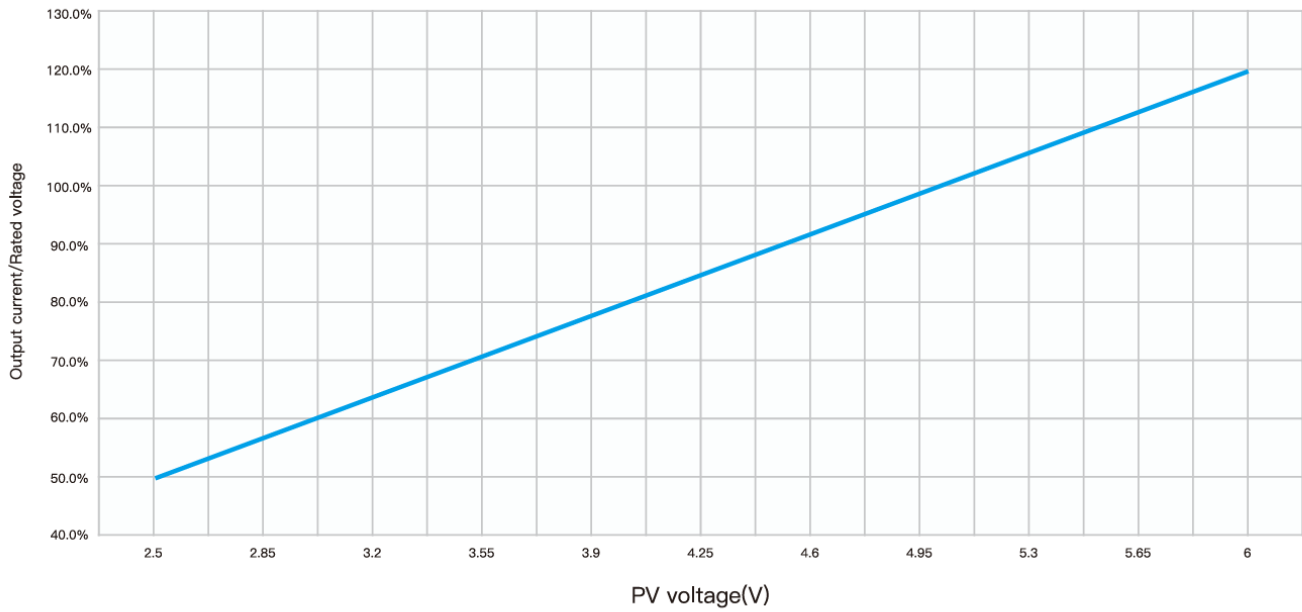
Output voltage vs PV voltage
