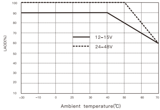
Derating curve (forced air cooling)
