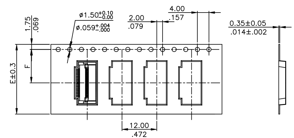
WIDTH : 16, 24 mm Carrier (SCALE 1:4)
